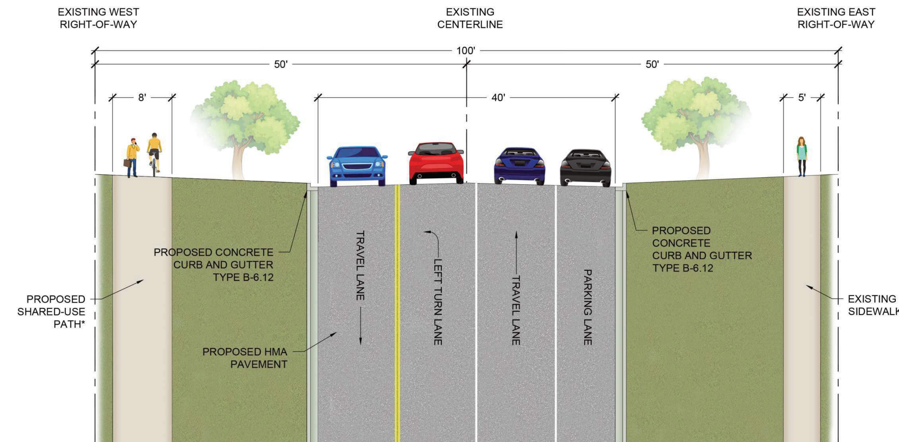
8' Shared Use Path (West Parkway)
