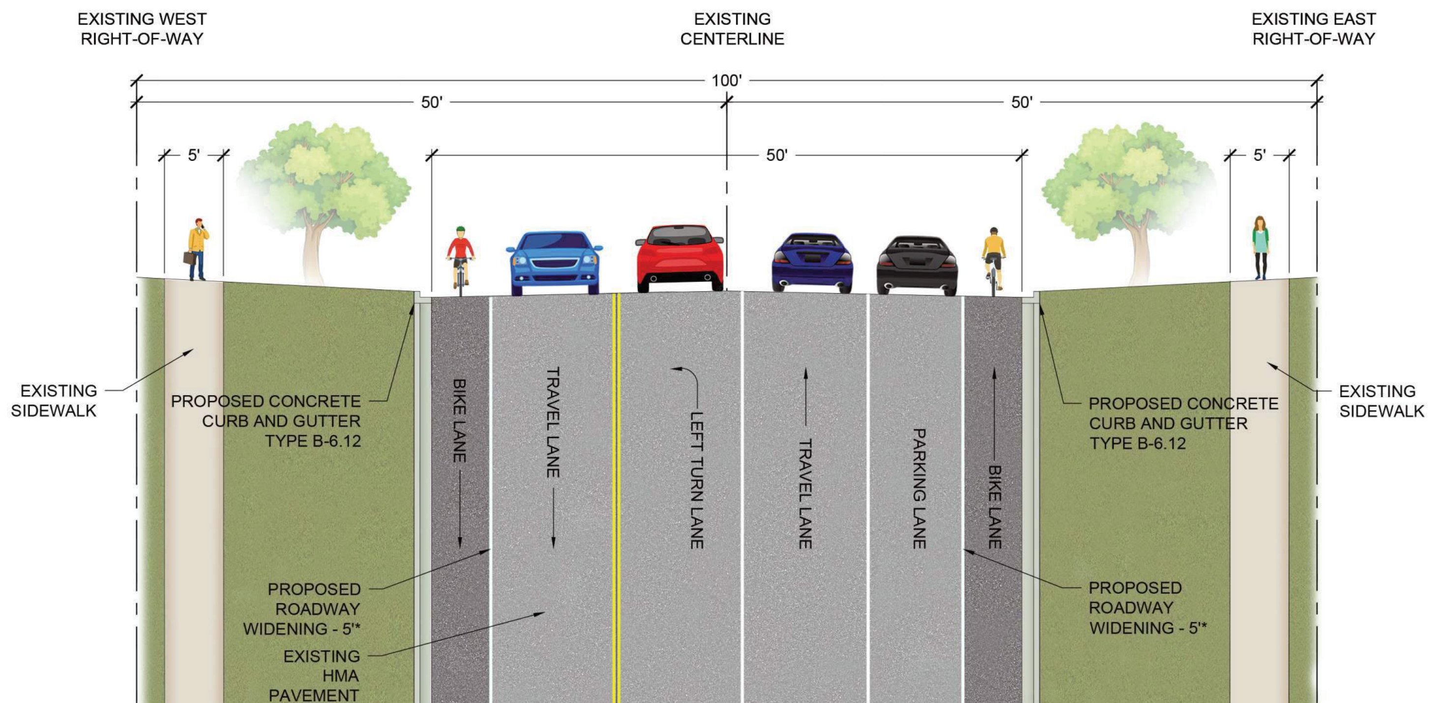
5' On Street Bike Lanes
