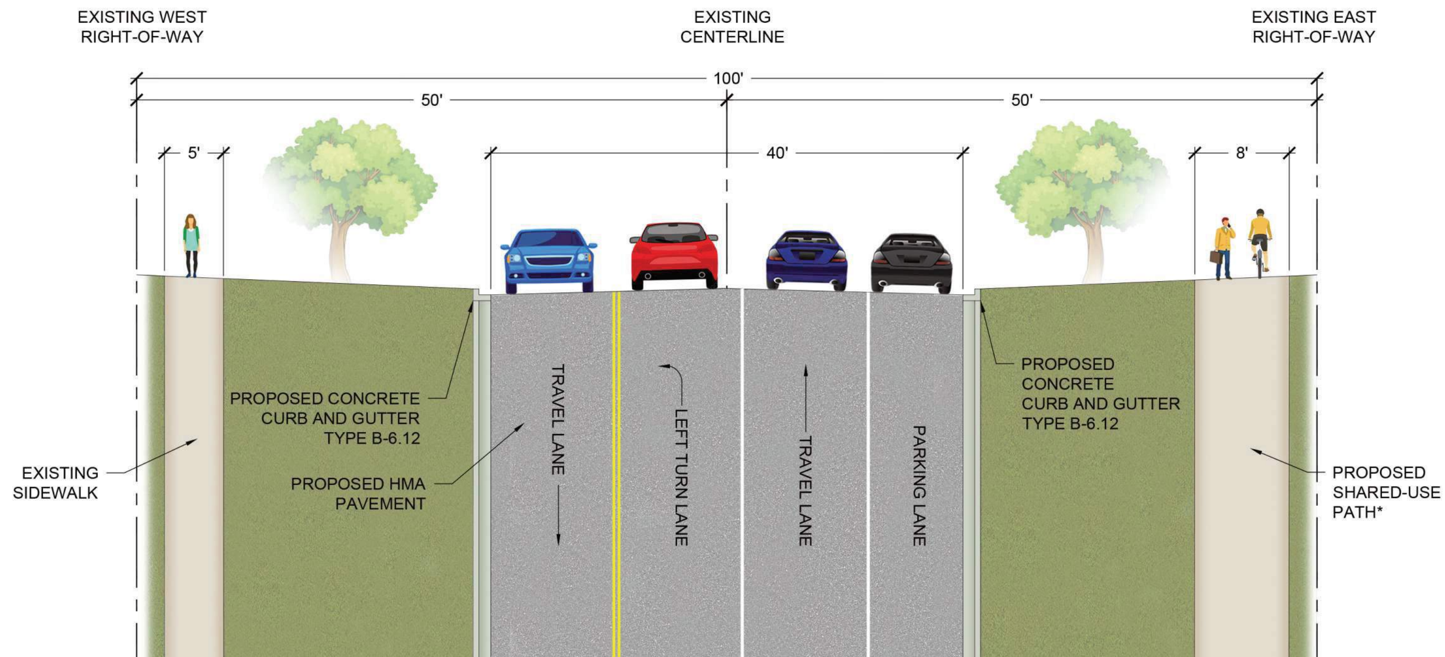
8' Shared Use Path (East Parkway)
